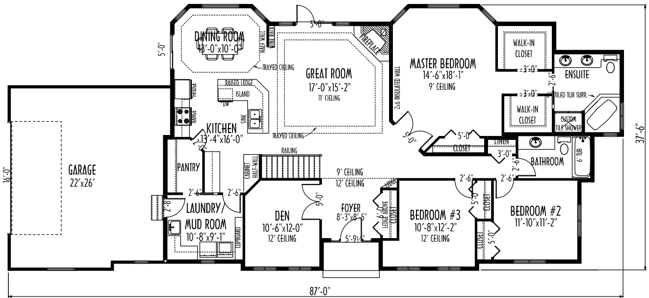
MAIN FLOOR PLAN AREA 2121 SQ. FT.
