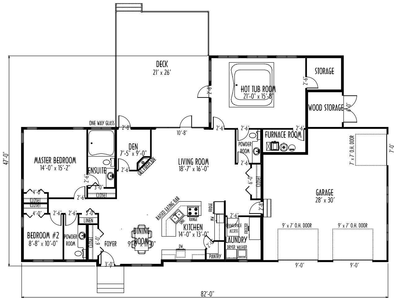
MAIN FLOOR PLAN 2111 SQ. FT.
