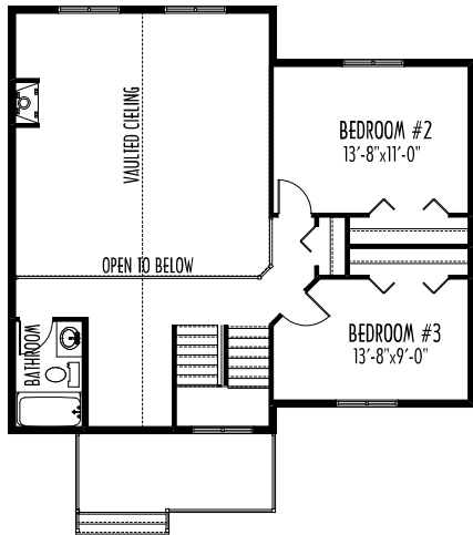
SECOND FLOOR PLAN 642 SQ. FT.
