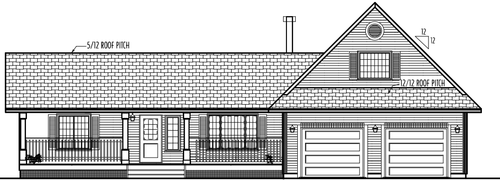
FRONT ELEVATION
