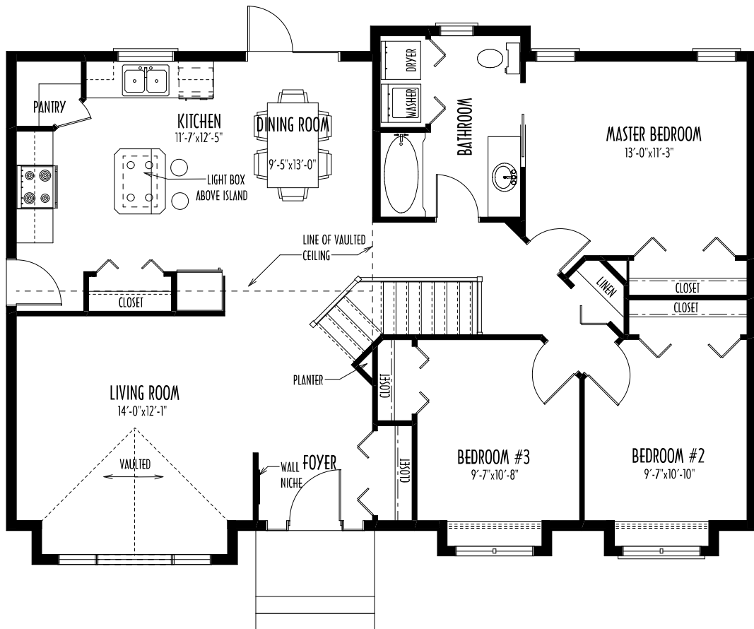
MAIN FLOOR PLAN AREA 1289 SQ.FT.
