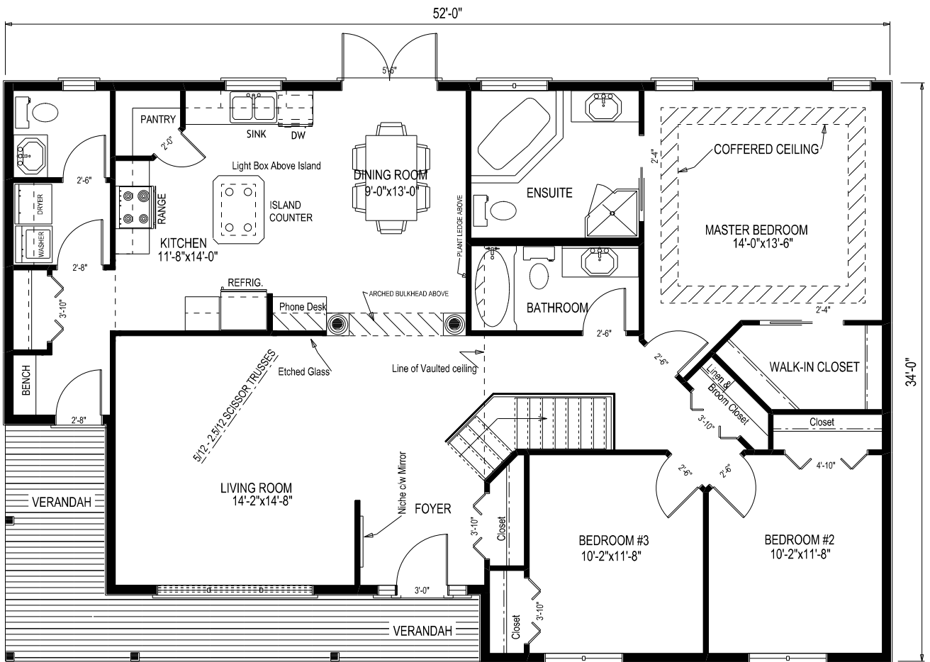
AREA 1596 SQ.FT. MAIN FLOOR PLAN
