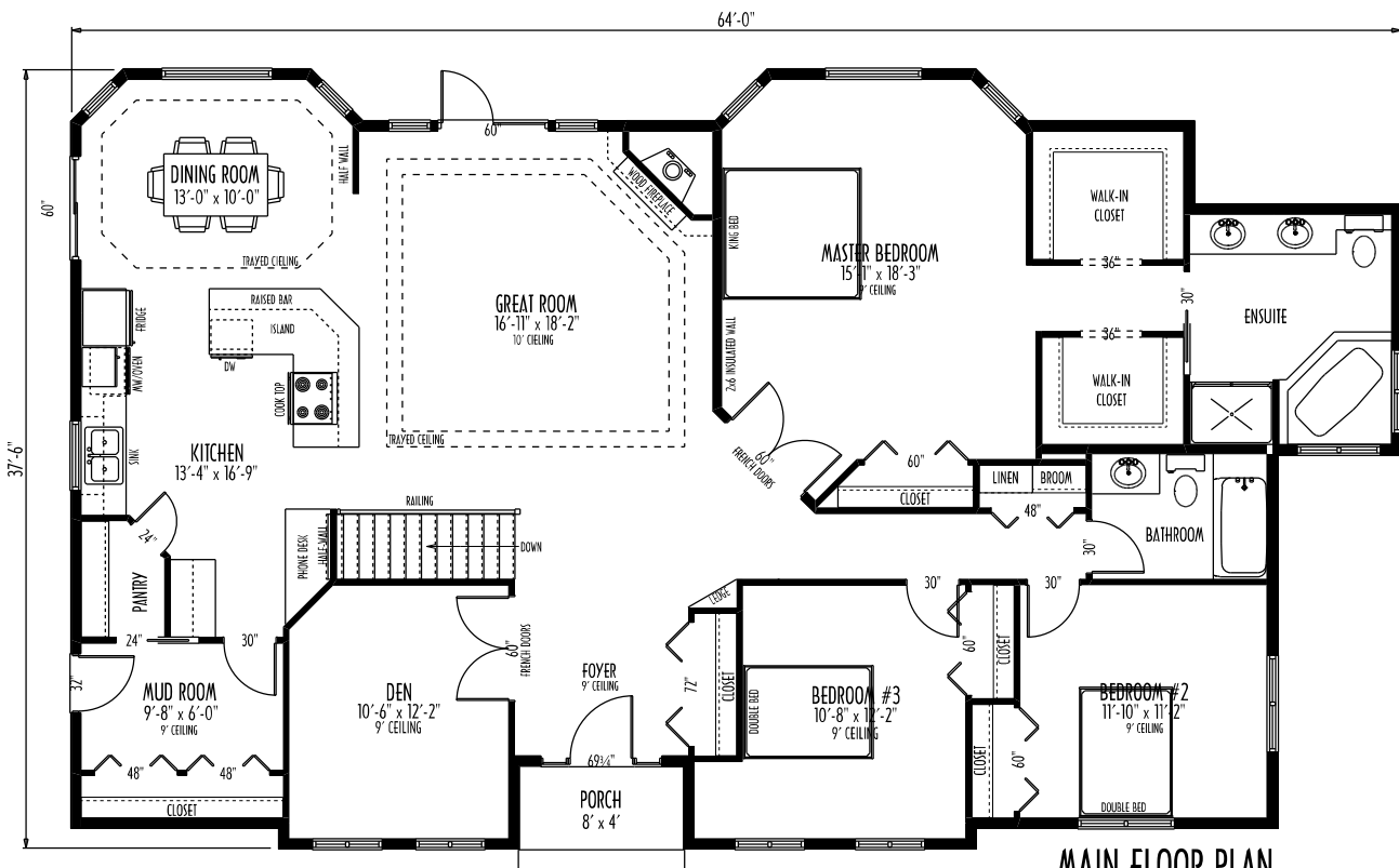
MAIN FLOOR PLAN AREA: 2090 SQ. FT.
