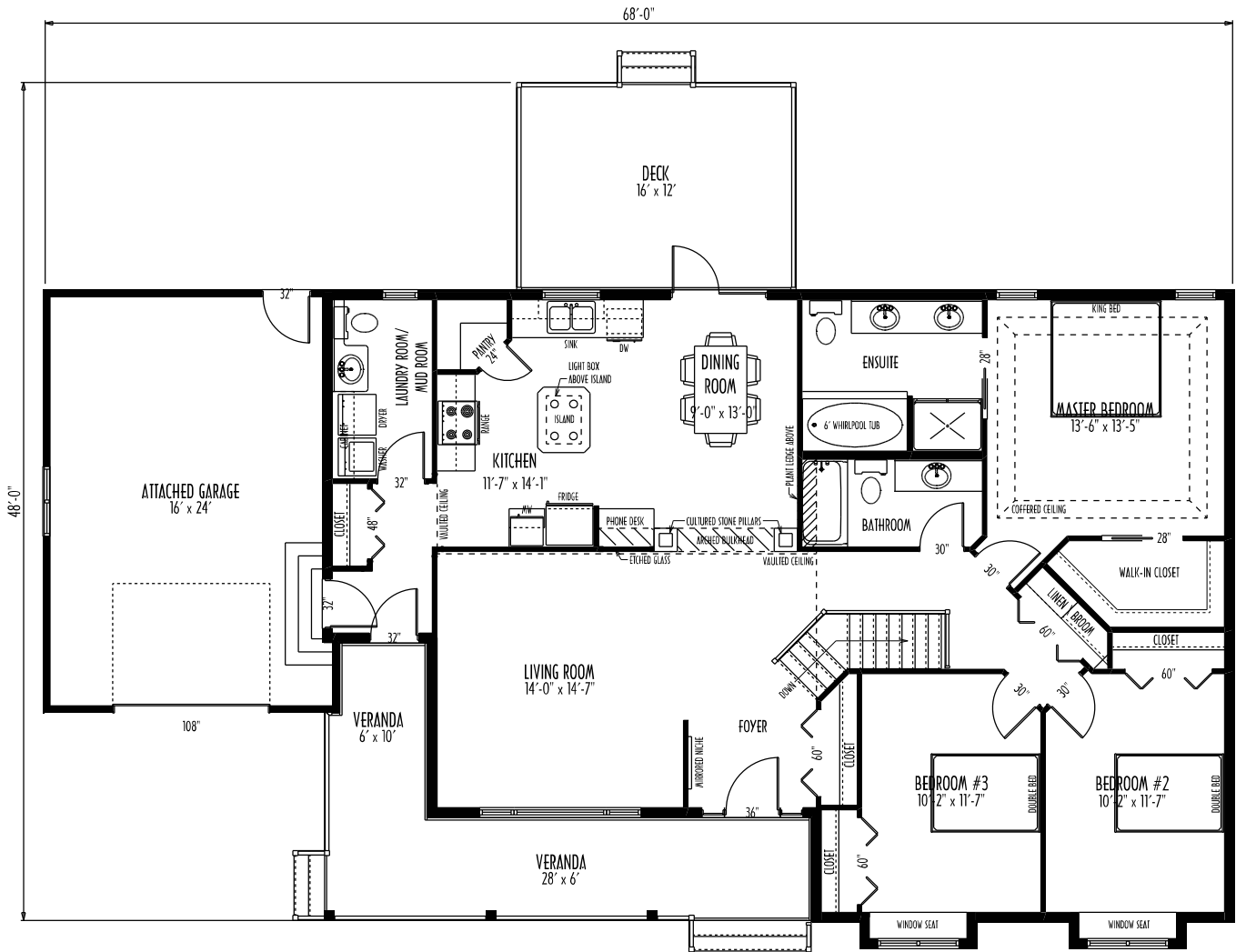
MAIN FLOOR PLAN AREA: 1664 SQ. FT.
