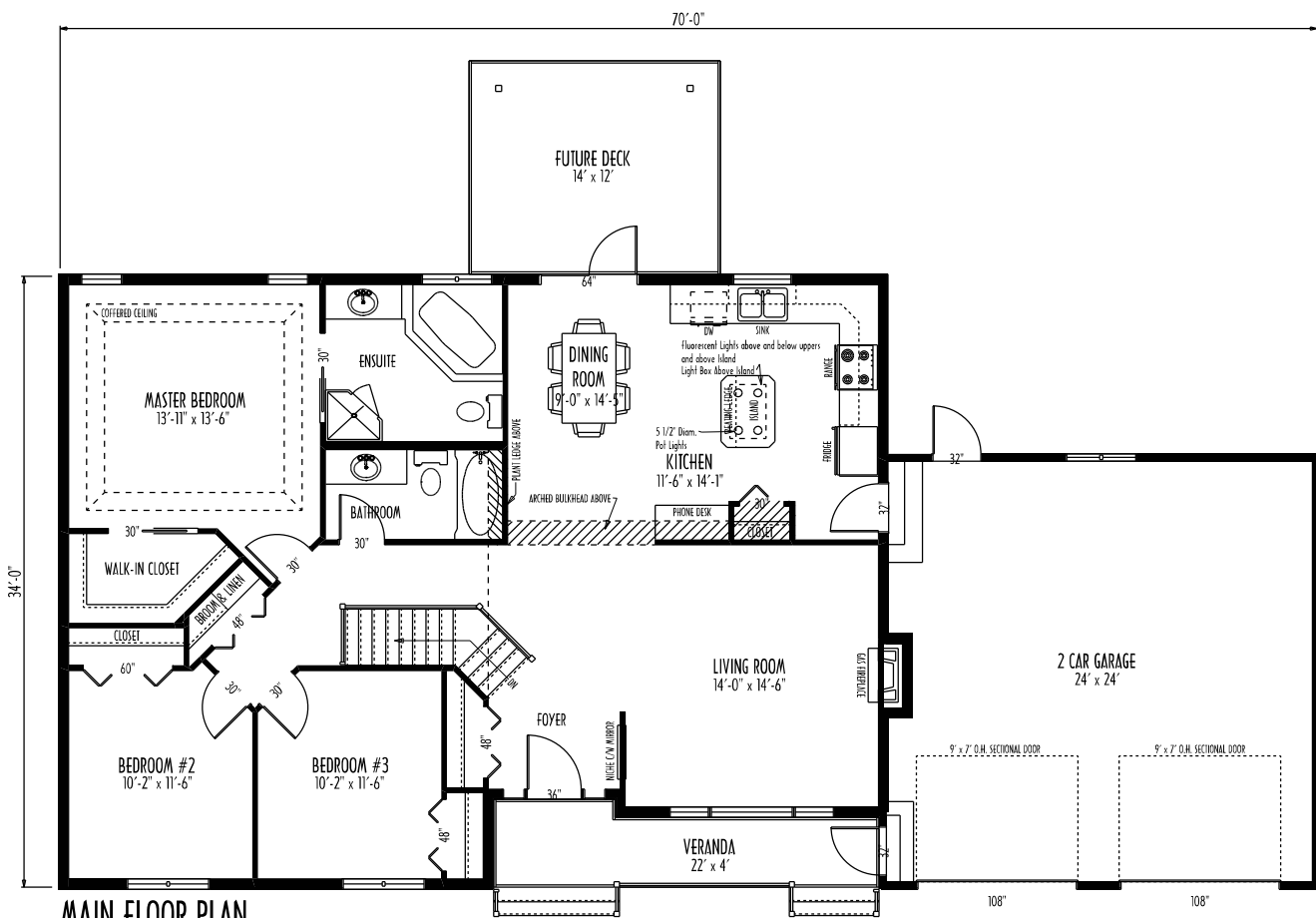
MAIN FLOOR PLAN AREA: 1475 SQ. FT.
