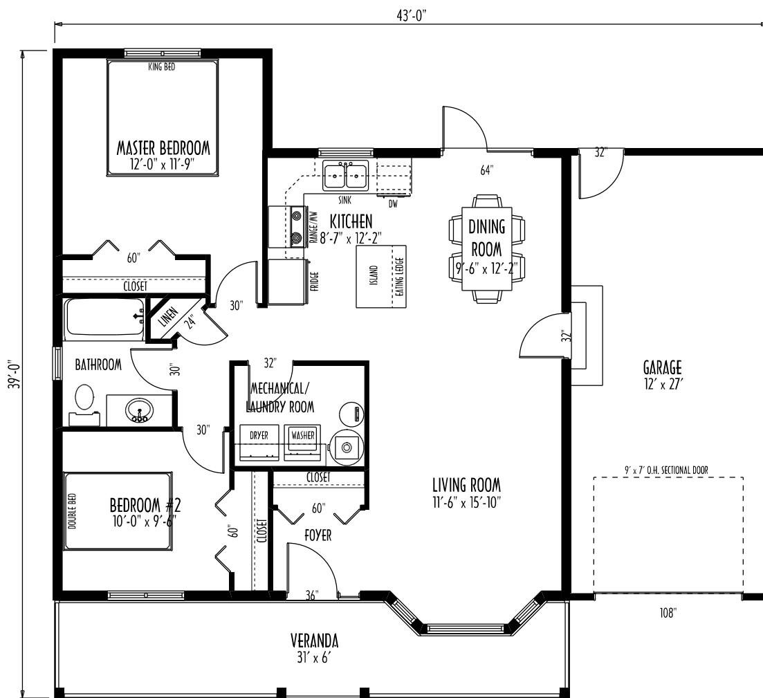
MAIN FLOOR PLAN AREA: 930 SQ. FT.
