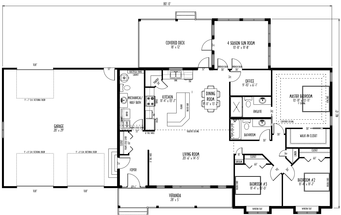
MAIN FLOOR PLAN TOTAL AREA: 1813 SQ. FT.
