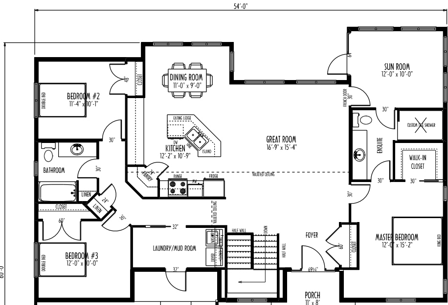
MAIN FLOOR PLAN AREA: 1687 SQ. FT.
