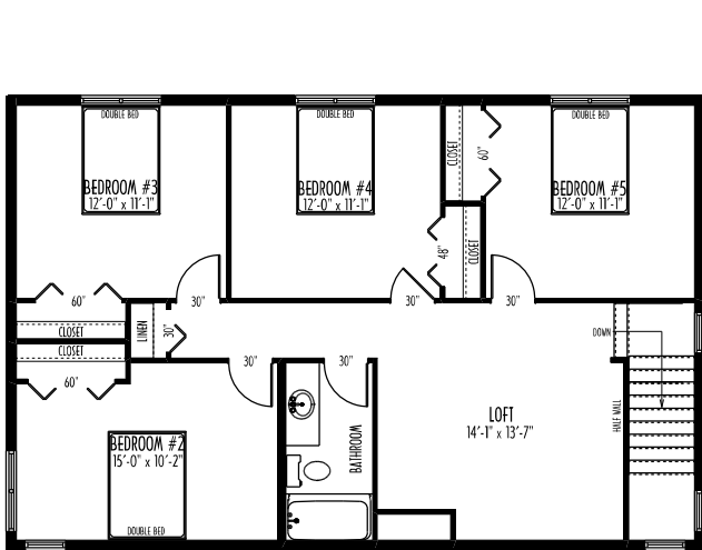
SECOND FLOOR PLAN AREA: 1040 SQ. FT.
