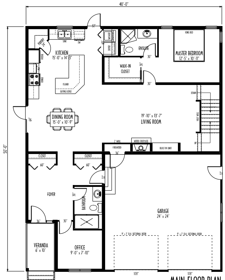
MAIN FLOOR PLAN AREA: 1364 SQ. FT.
