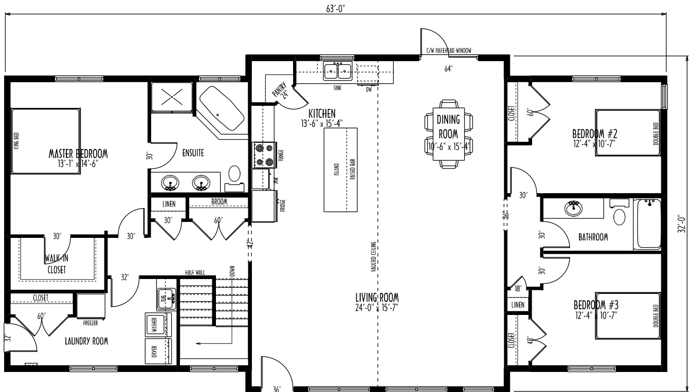
MAIN FLOOR PLAN AREA: 1864 SQ. FT.
