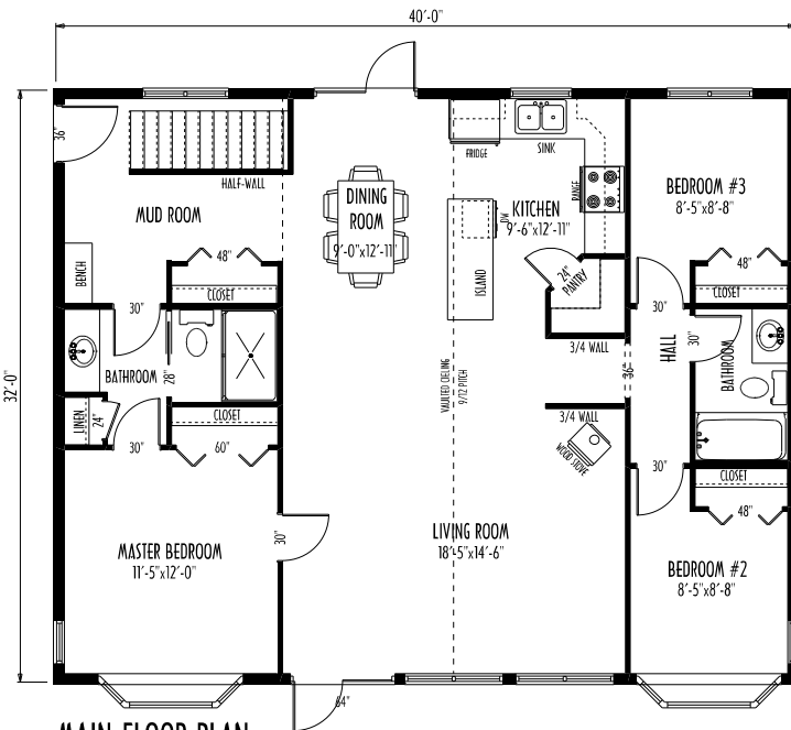
MAIN FLOOR PLAN AREA: 1297 SQ. FT.
