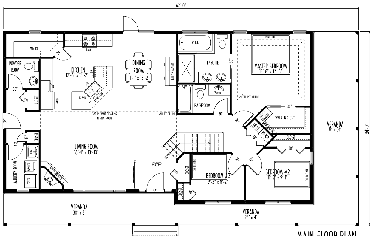
MAIN FLOOR PLAN AREA: 1560 SQ. FT.
