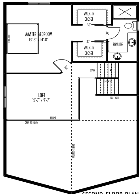
SECOND FLOOR PLAN AREA: 609 SQ. FT.
