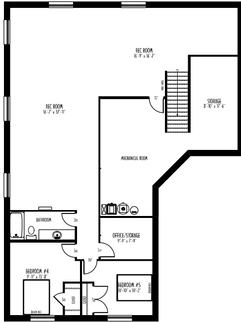
BASEMENT LAYOUT
