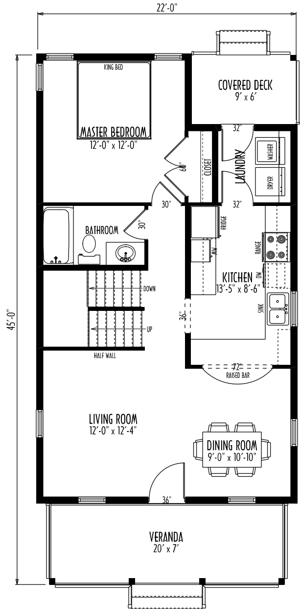
MAIN FLOOR PLAN AREA: 782 SQ. FT.
