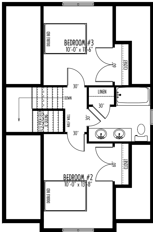
SECOND FLOOR PLAN AREA: 486 SQ. FT.
