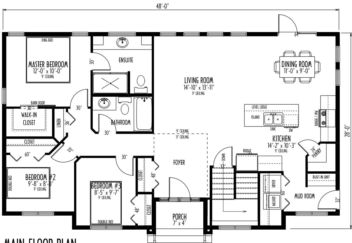
MAIN FLOOR PLAN AREA: 1281 SQ. FT.
