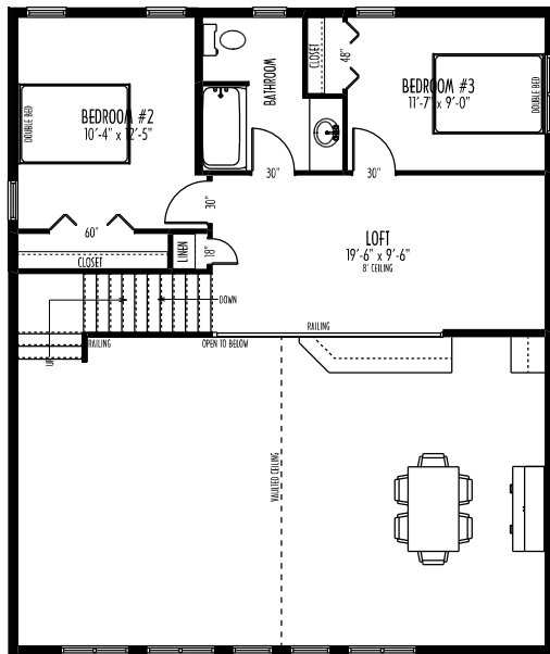
SECOND FLOOR PLAN AREA: 567 SQ. FT.
