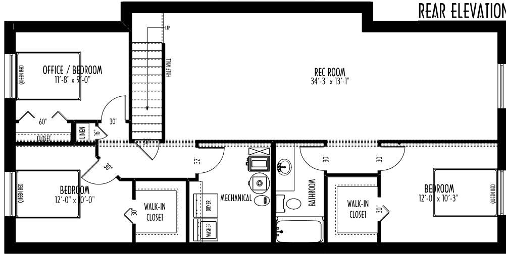
BASEMENT PLAN AREA: 1300 SQ. FT.
