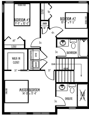
SECOND FLOOR PLAN AREA: 731 SQ. FT.
