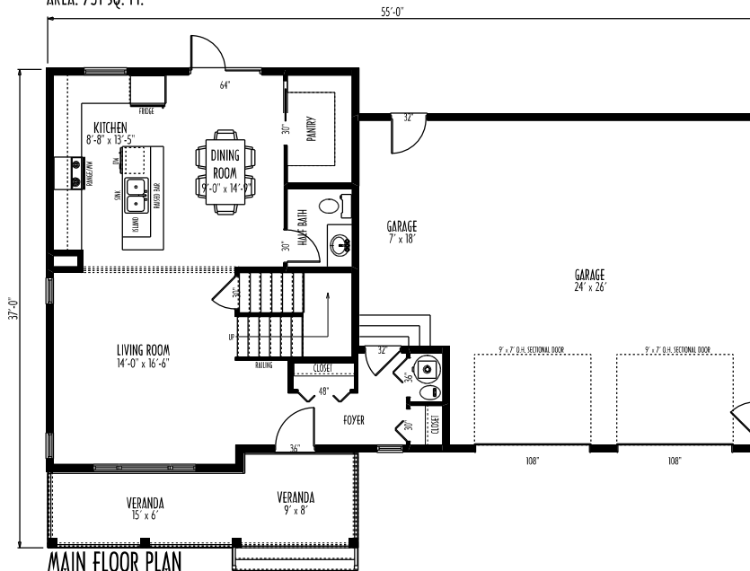
MAIN FLOOR PLAN AREA: 787 SQ. FT.
