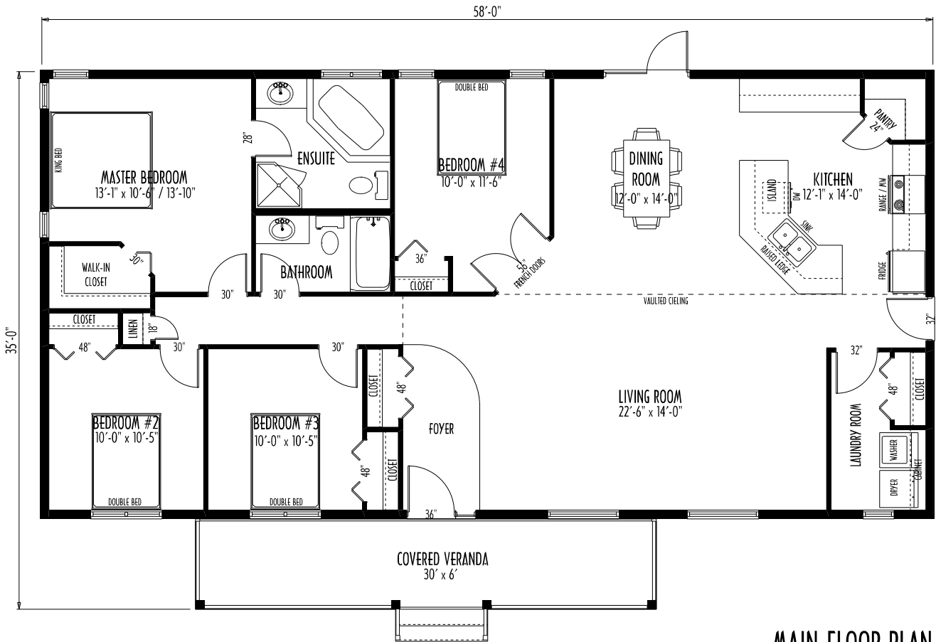
MAIN FLOOR PLAN AREA: 1682 SQ. FT.
