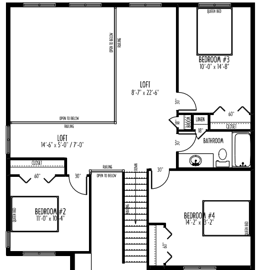
SECOND FLOOR PLAN AREA: 901 SQ. FT.
