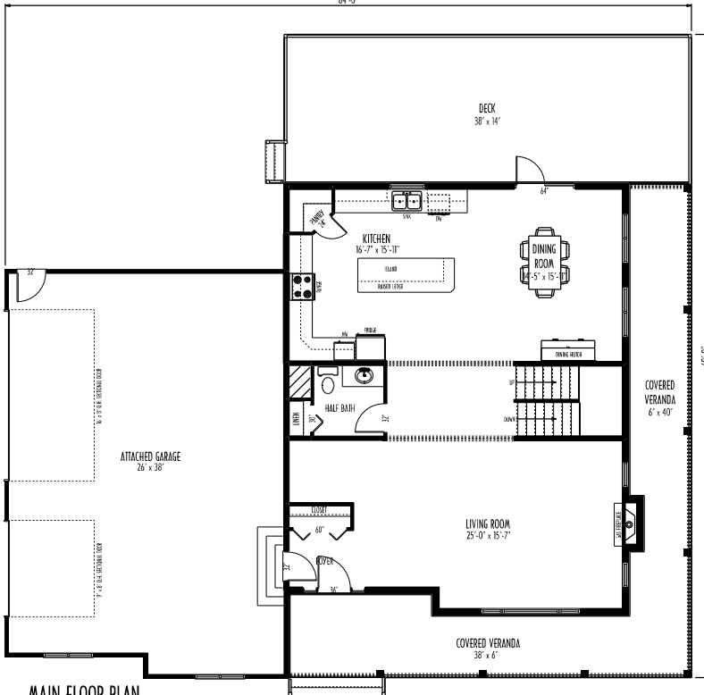
MAIN FLOOR PLAN AREA: 1258 SQ. FT.
