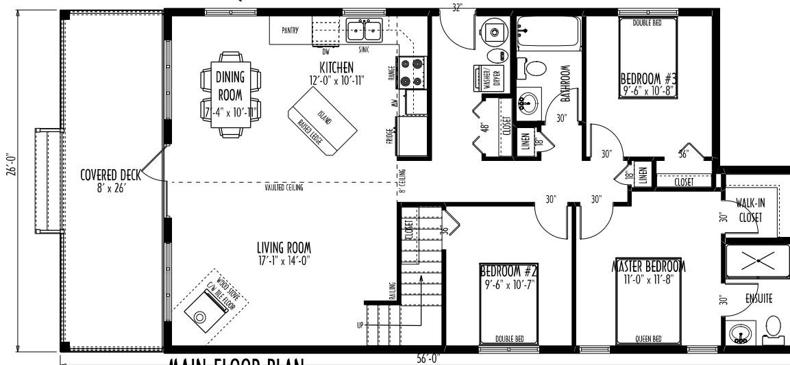
MAIN FLOOR PLAN AREA: 1176 SQ. FT.
