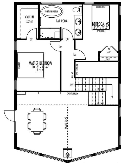
SECOND FLOOR PLAN AREA: 601 SQ. FT.
